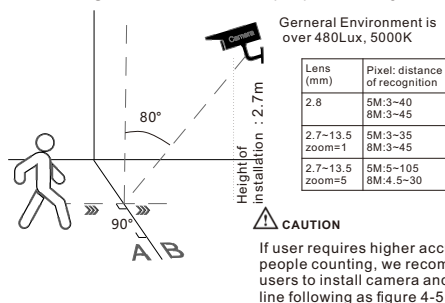
Figure 4-4 Installation of people counting
