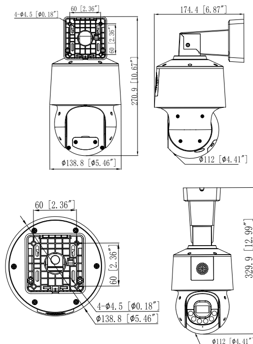
Figure 2-5 Dimensions of Dome(Unit:mm)
